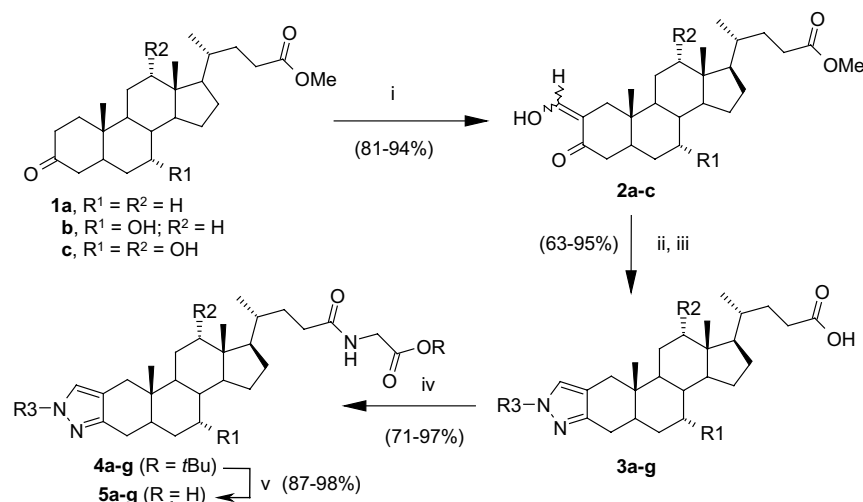
Scheme 1. Reagents and conditions: (i) NaH/HCO 2 Et/cat. EtOH/toluene, rt, 12–24 h; (ii) H 2 NNHR 3 /EtOH, reflux, 8–12 h; (iii) 2 N NaOH/THF, rt, 5–8 h; (iv) EDAC/H–Gly–OBu–tHCl/DIEA/DCM, rt, 12–18 h; (v) 4 M HCl in dioxane, rt, 5–8 h.
